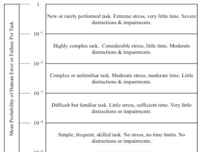
Figure 4 Generic human error rates 7 (redrawn)
